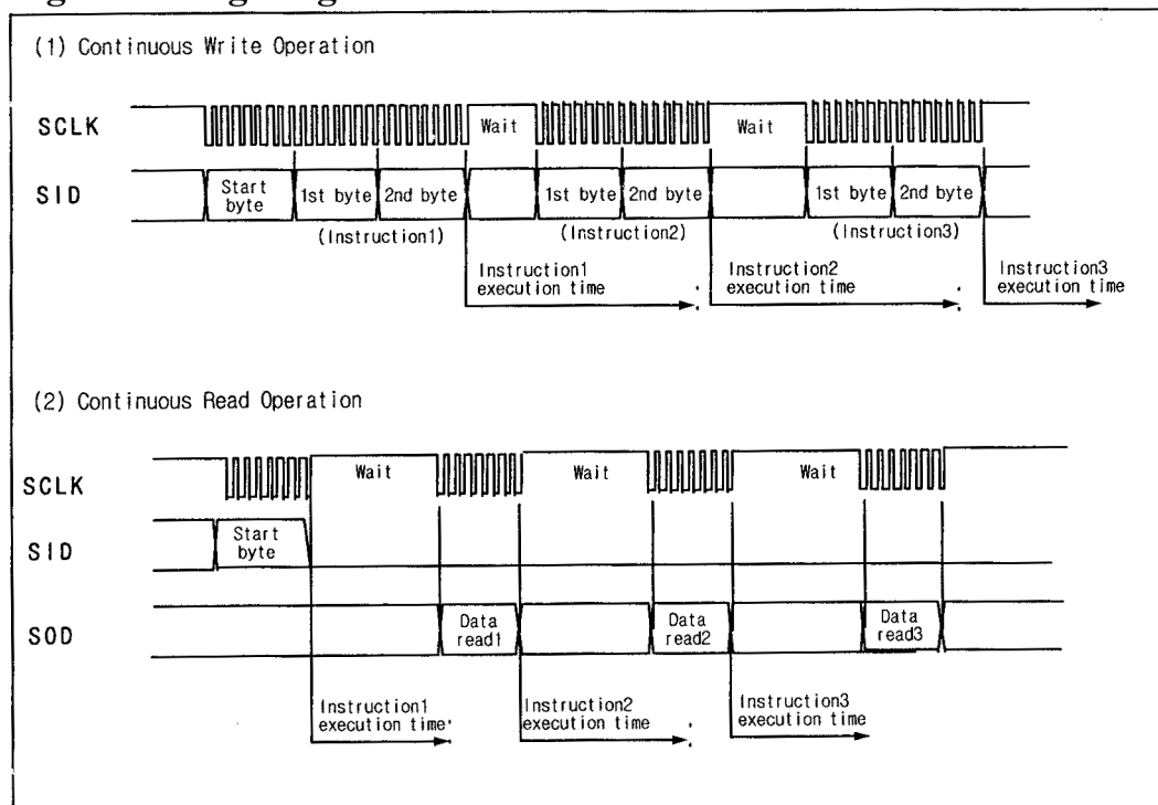
Fig.14 Timing Diagram of Continuous Data Transfert
