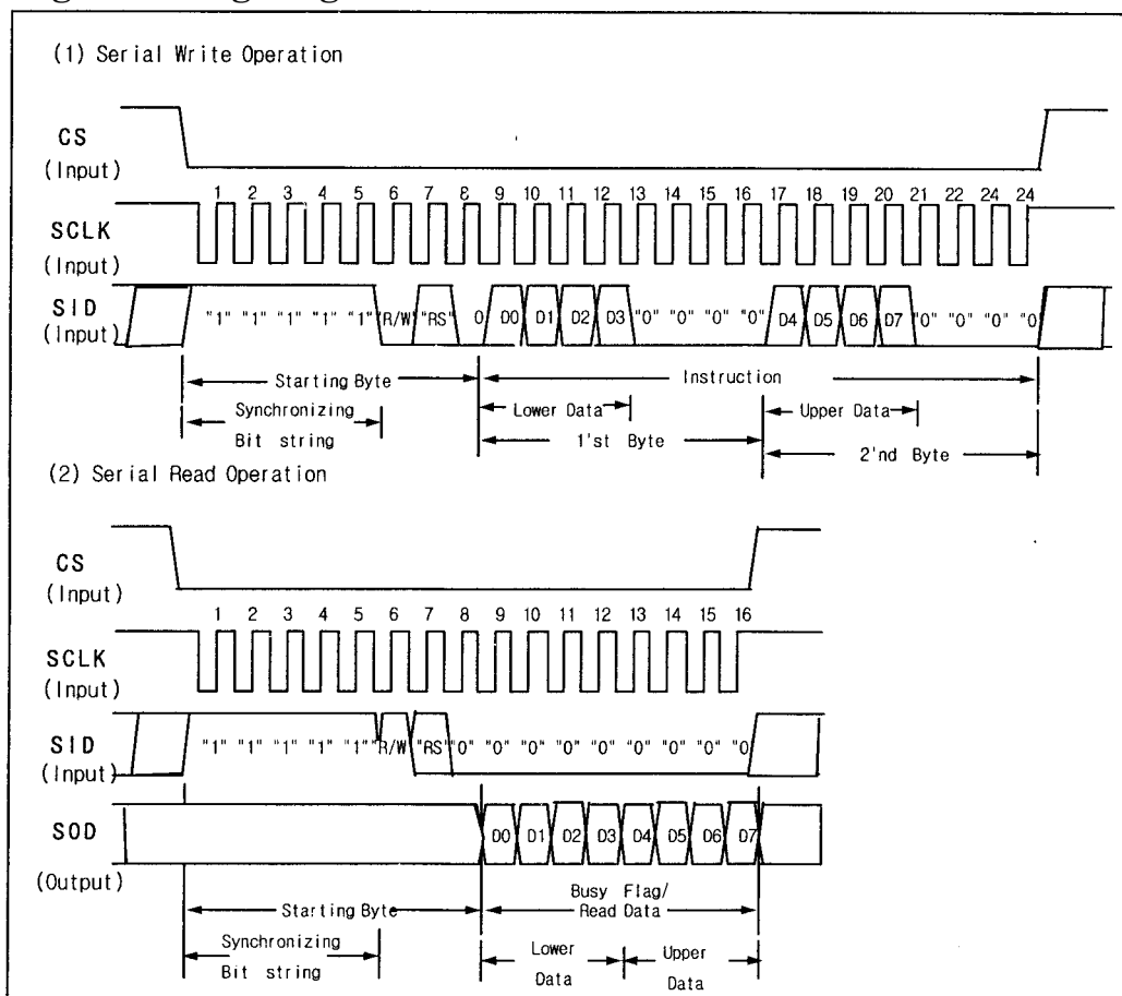
Fig.13 Timing Diagram of Sérial Data Transfert
